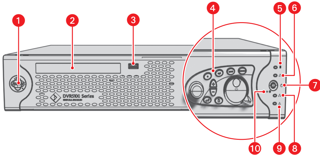
Figure 55. DVR5100 Front Panel Indicators
